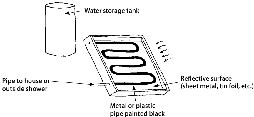
Solar water heater placed in the sun on a roof or at ground level
