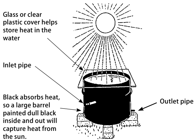
A simple water heater
